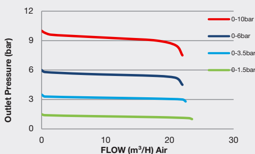
25 bar Inlet Pressure @ 21°C
